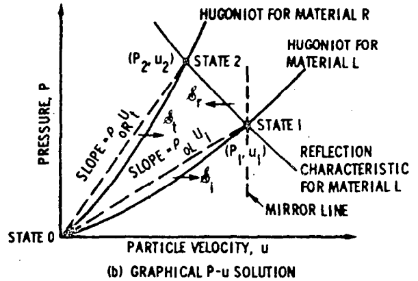
(b) GRAPHICAL P-u SOLUTION
